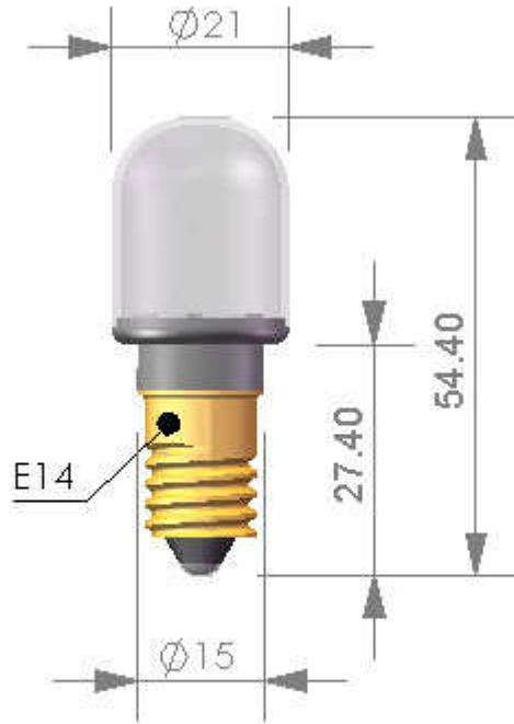
(T5)E14 5SMD
